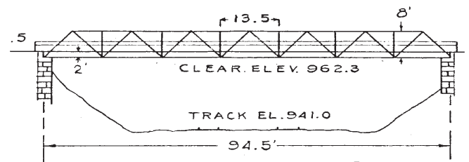
LIVERMORE R.R. OVERPASS 1 SPAN STEEL PONY TRUSS, WOOD FLOOR STONE ABUTMENTS - 28', PIPE RAILING OVERALL WIDTH 23', ROADWAY 18.5' SCALE: 1" = 30'
